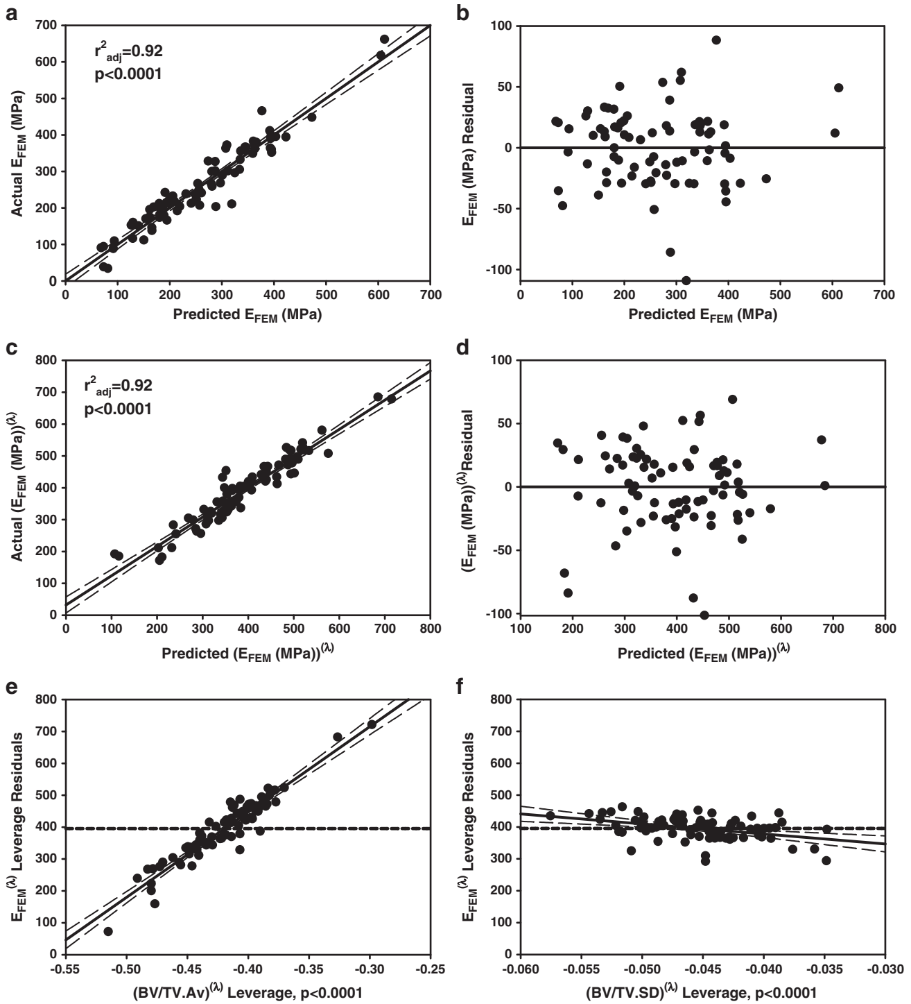
Fig. 1. a) E_{FEM} calculated from finite element models vs E_{FEM} predicted by the multiple regression model including BV/TV.AV and BV/TV.SD using nontransformed variables. b) The residuals for the model with nontransformed variables. c) As in 1a except using transformed variables. d) The residuals for the model with transformed variables. e) Leverage plot for BV/TV.AV and f) Leverage plot for BV/TV.SD. Solid, medium dashed and small dashed lines show linear fits, 95% confidence intervals and mean of the actual E_{FEM} , respectively. (95% confidence curve crossing the mean response line indicates a significant leverage for the effect.) The model with transformed variables and that with nontransformed variables were qualitatively similar.
